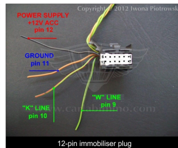
12-pin immobiliser plug
