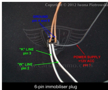
6-pin immobiliser plug
