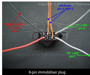
8-pin immobiliser plug
