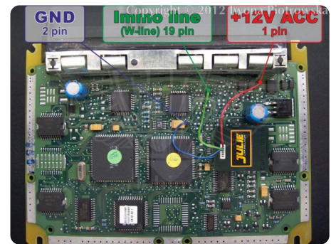
Although the picture shows Julie Emulator, the same way of connecting to ECU also applies to Clixe
