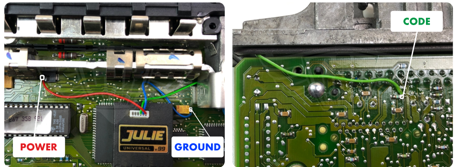
Although the picture shows Julie Emulator, the same way of connecting to ECU also applies to Clixe
