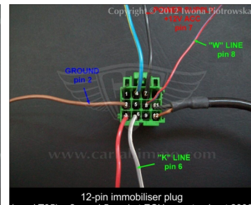
12-pin immobiliser plug (e.g. LT35) – 2 - and 5-socket ECUs up to about 2006
